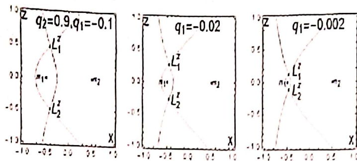
Fig.5. Zero velocity curves in the (x, z) plane and locations of the out of plane equilibria for q_1 = -0.1 , q_1 = -0.02 and q_1 = -0.002 correspondingly. The locations of the primary bodies are presented too. Note: The value of \mu = 0.5 , and q_2 = 0.9 are fixed for all cases
