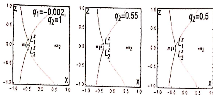
Fig.6. Zero velocity curves in the (x, z) plane and locations of the out of plane equilibria for q_2 = 1 , q_2 = 0.55 and q_2 = 0.5 correspondingly. The locations of the primary bodies are presented too. Note: The value of \mu = 0.5 , and q_1 = -0.002 are fixed for all cases
