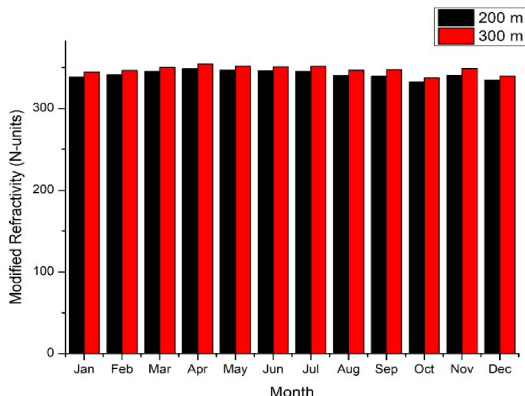
Figure2: Monthly variation of modified refractivity at heights of 200 m and 300 m.
