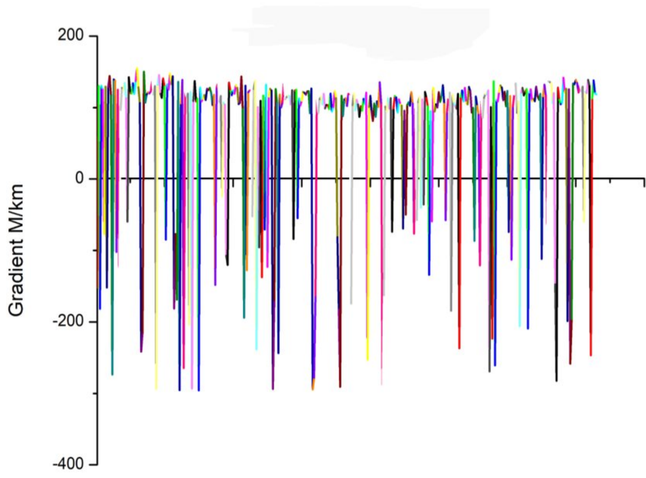
Figure 3: Daily variation of vertical gradients.
