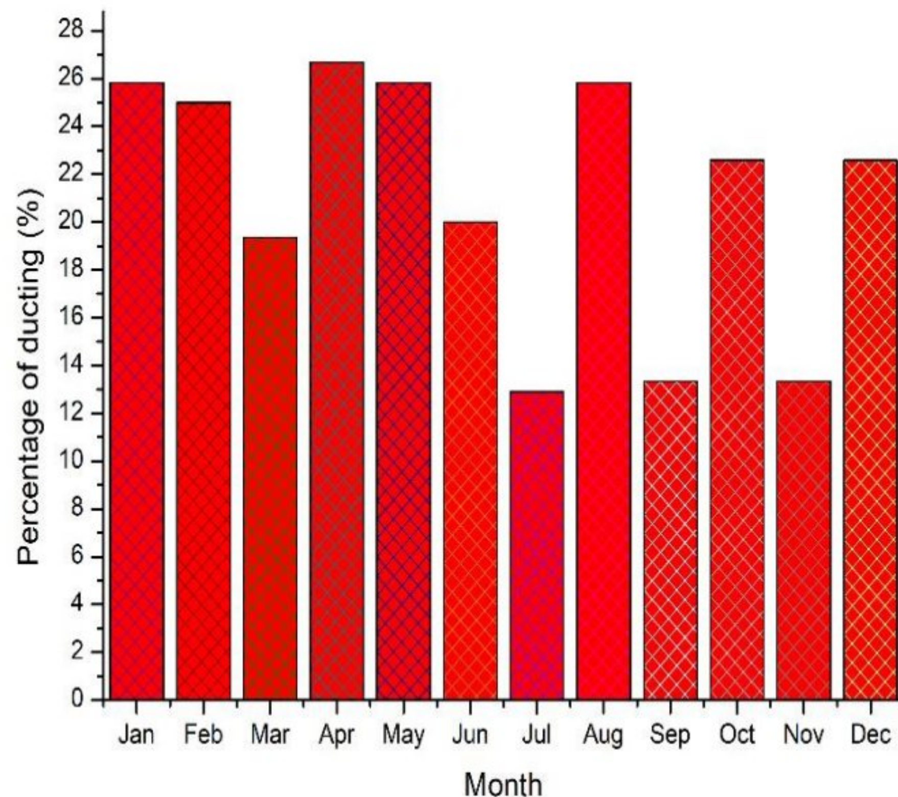
Figure 5: The monthly percentage occurrence of atmospheric ducting
